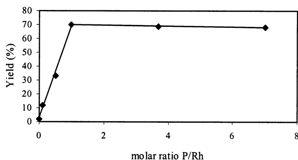
Fig. 4. Influence of added triphenylphosphine on the rate of hydroformylation with [\text{Rh}_2(\mu\text{-S}'\text{Bu})_2(\text{CO})_2(\text{TPPTS})_2] .
