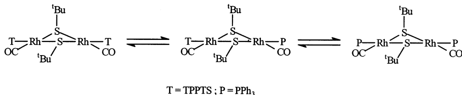
Fig. 3. Ligand exchange equilibria between the two phosphine ligands in the dinuclear complexes.
