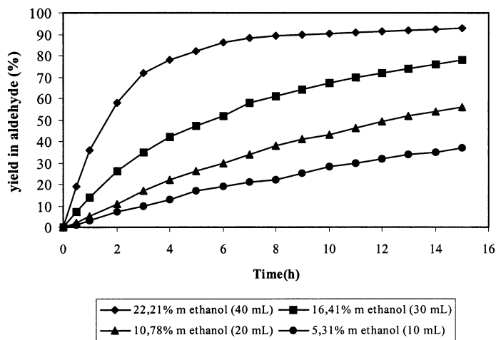
Fig. 2. Influence of the quantity of ethanol on the yield in C 9 aldehydes vs. time.
